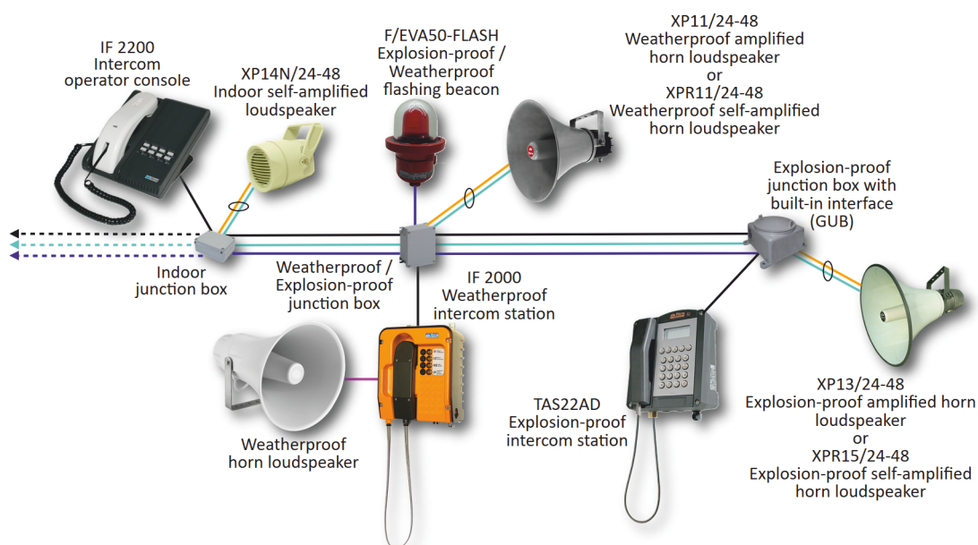
New IF 2000 Public Address & Intercom with Analog Intercom Stations
