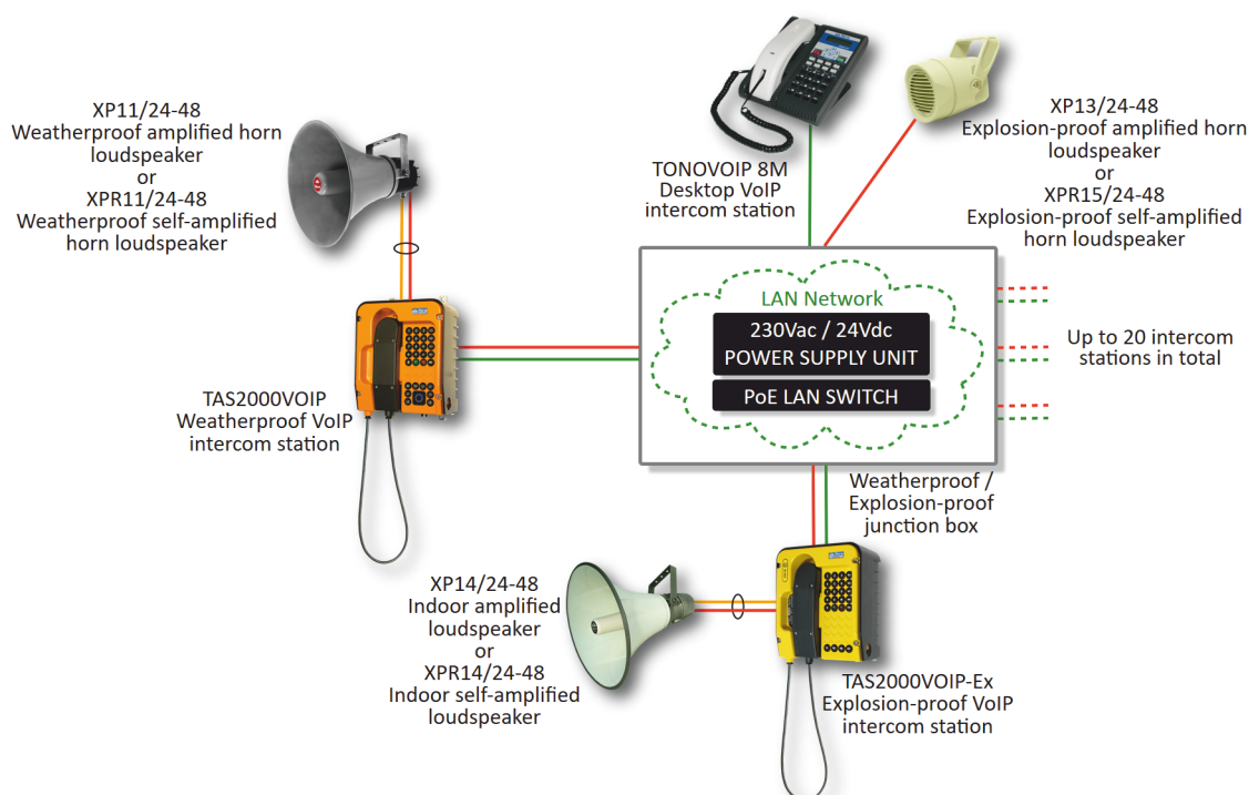
ASTROLess Public Address & Intercom with VoIP Intercom Stations
